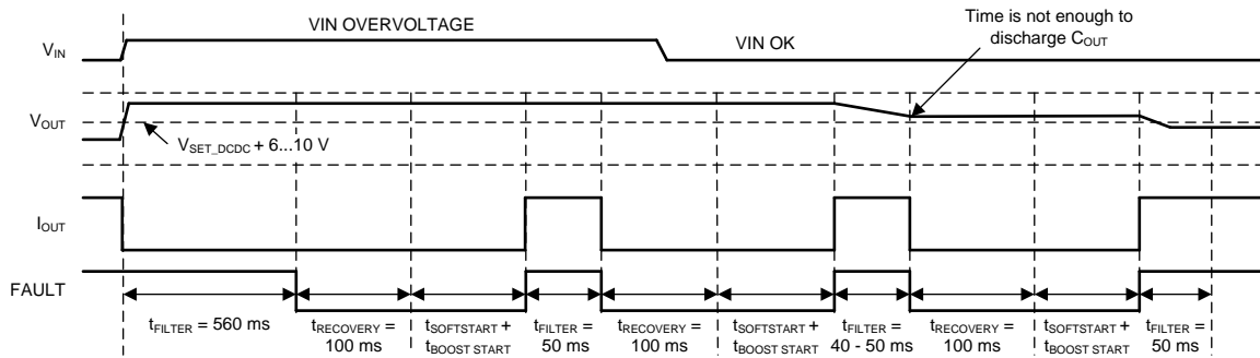
Figure 11. V_{IN} Overvoltage Protection (DC-DC OVP)
