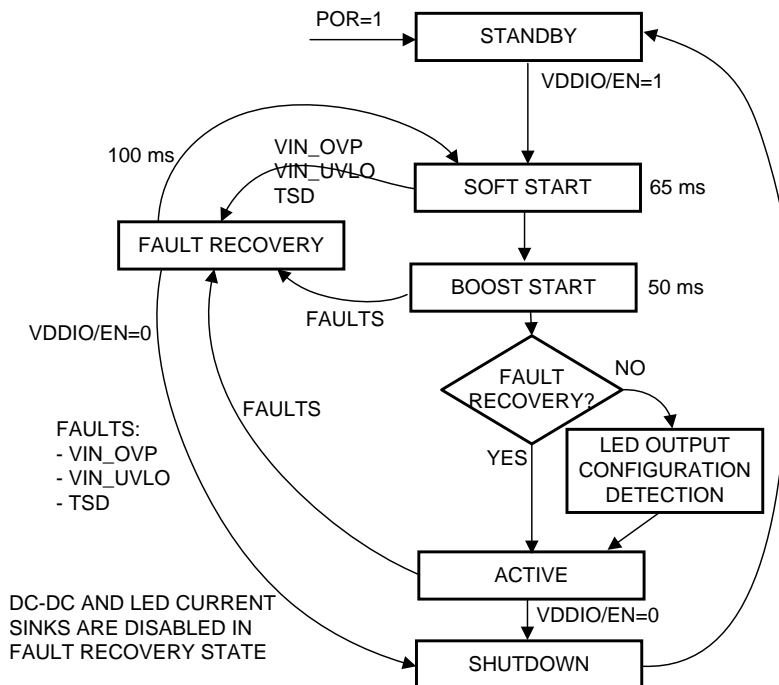
Figure 16. State Diagram
